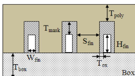
Figure 1: Structure of a three-fin (n=3) SOI-FinFET
