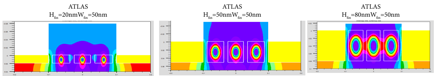
Figure 5: Potential in the oxide and the silicon in the y-z section for the three fin Dual-gate SOI-FinFET; ( V_{gs}=0.5V )
