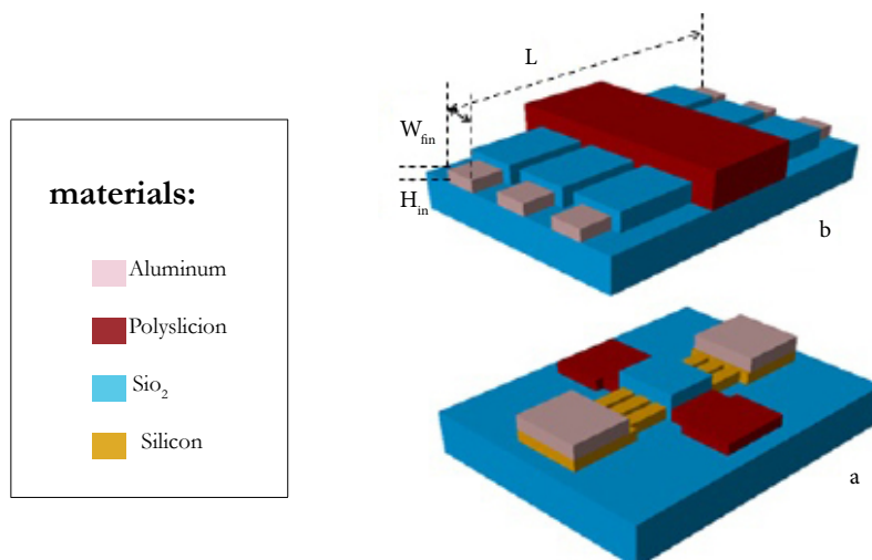
Figure2: 3D structure of a three-fin (n=3) Dual-gate SOI-FinFET (a); Tri-gate SOI-FinFET (b)
