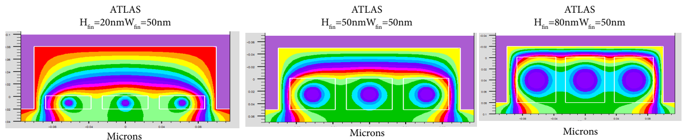
Figure 4: Potential in the oxide and the silicon in the y-z section for the three fin tri-gate SOI-FinFET; ( V_{gs}=0.5V )
