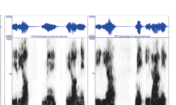
Figure 32: Shows the Spectrogram of Mother & Daughter for word "syria me iran"
