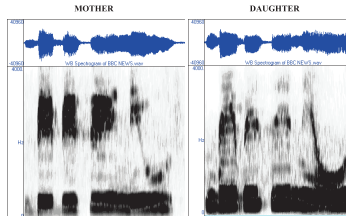
Figure 51: Shows the Spectrogram of Mother & Daughter for word "BBC news"
