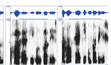
Figure 55: Shows the Spectrogram of Mother & Daughter for word "kaha hai ki unka desh"
